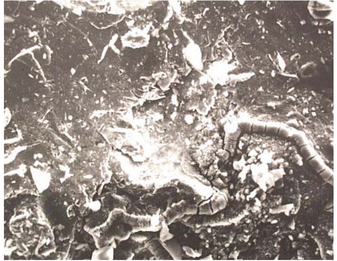
Surface profile showing contaminants and shattered abrasive particles impregnated into the metal profile at this magnification level
